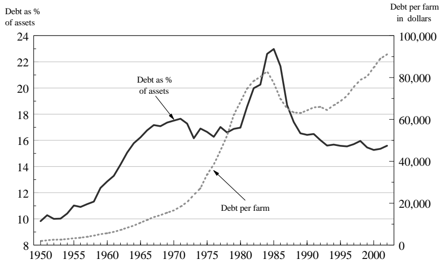
Figure 5. Farm debt as a percent of farm assets and farm debt per farm in the U.S., 1950-2002.
