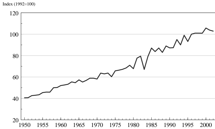
Figure 1. Total factor productivity in U.S. agriculture, 1950-2002.
