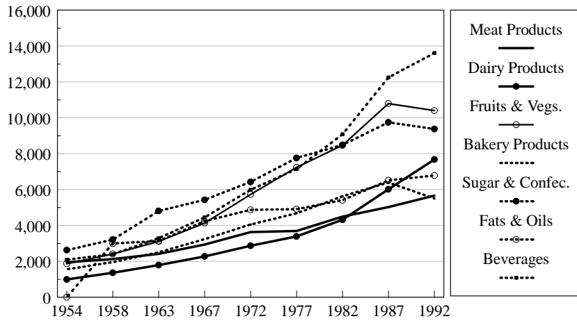
Figure 10. Real value added per establishment in U.S. food-processing, 1954-92.
