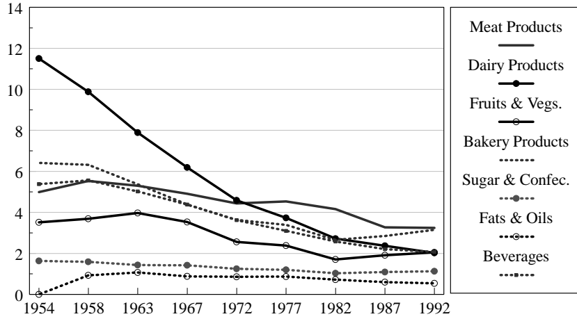
Figure 9. Number of establishments in U.S. food-processing, 1954-92.
