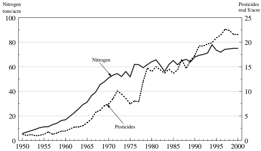
Figure 7. Nitrogen and pesticide use per acre planted in the U.S., 1950-2000.
